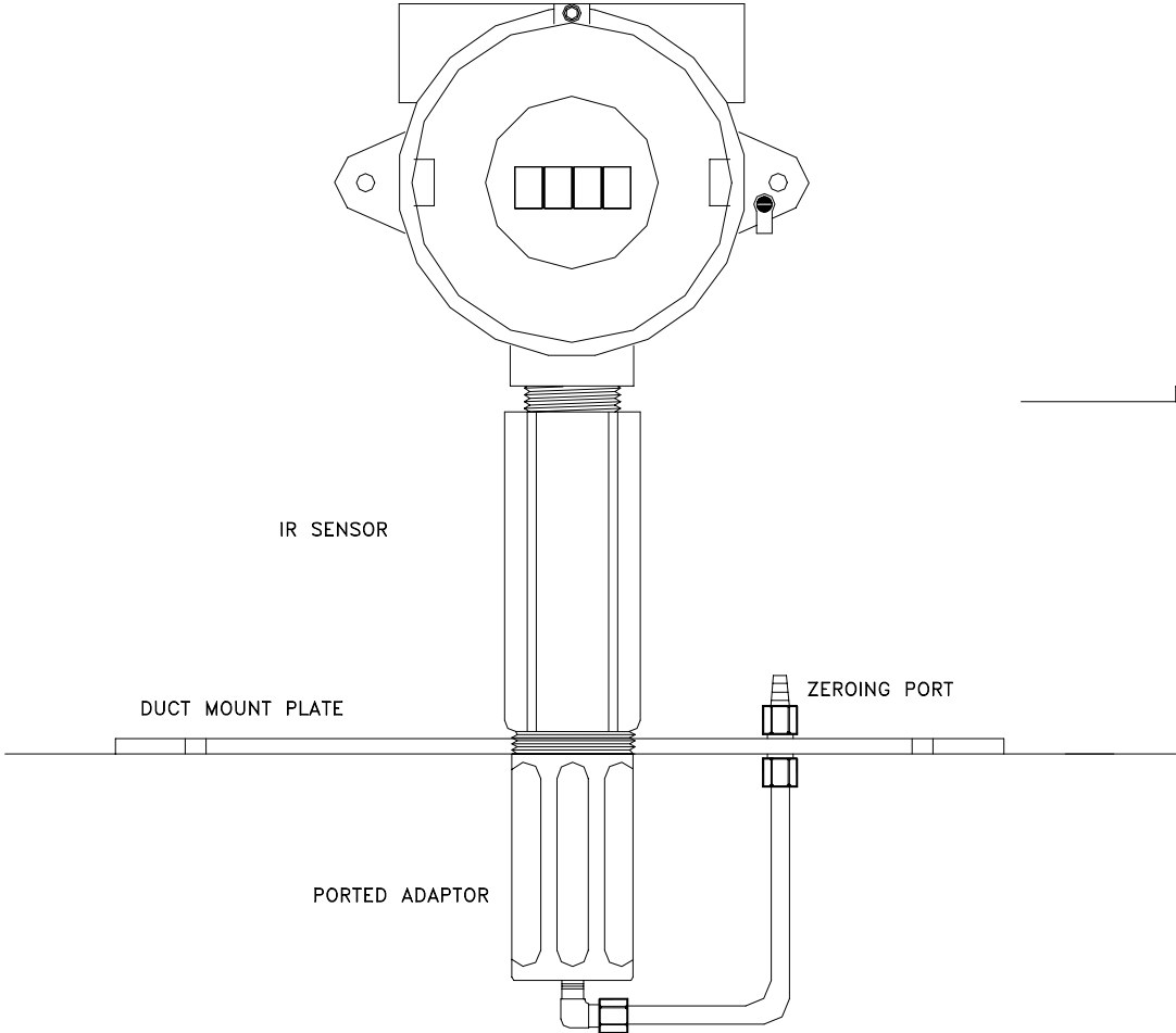
IR DUCT MOUNTING PLATE 361-248-02
