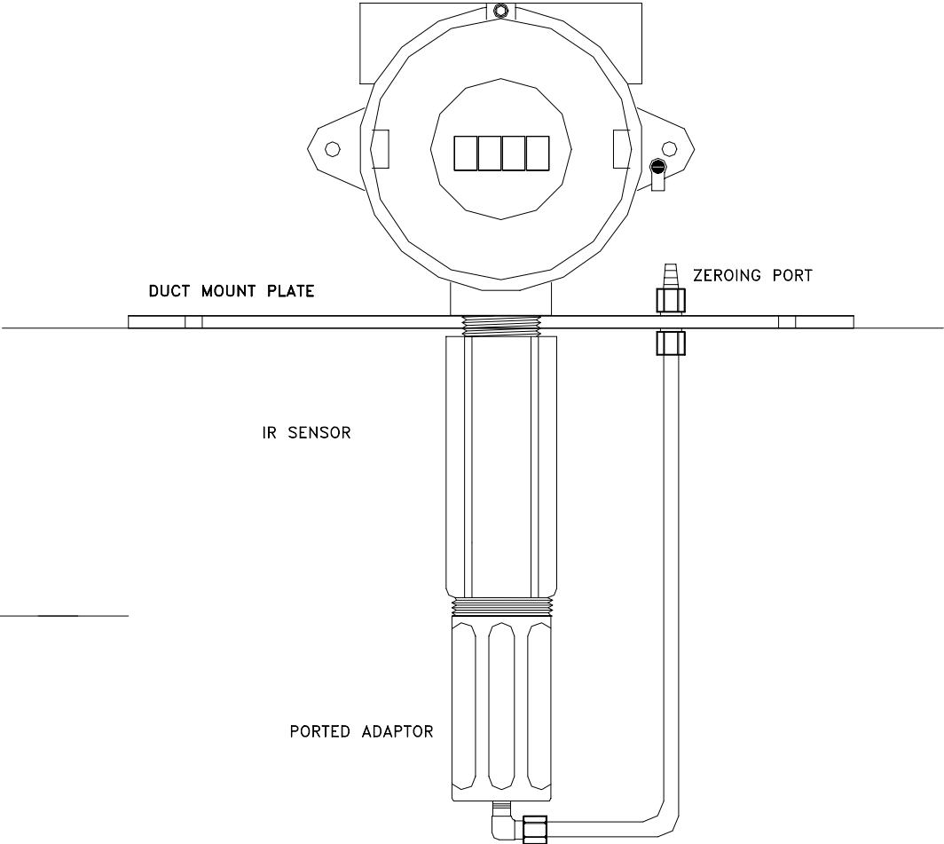
IR DUCT MOUNTING PLATE 361-248-01
